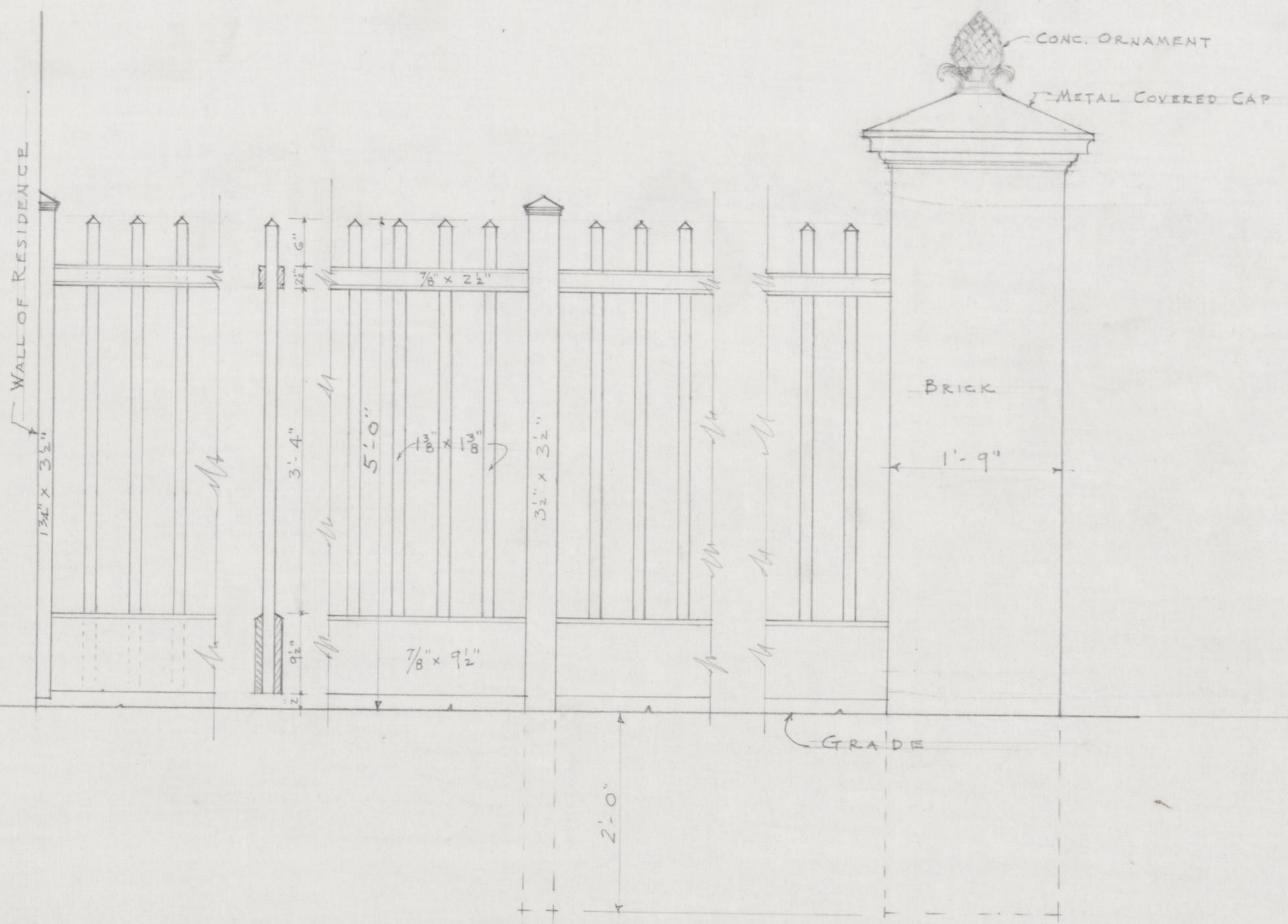
ELEVATION SCALE 3/4" = 1' - 0"
